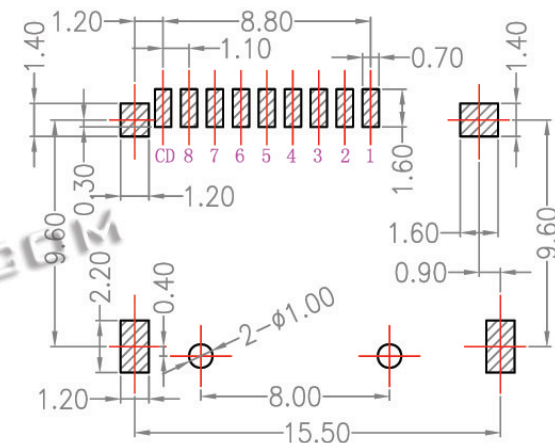
P.C.B LAYOUT (TOLERANCE: ±0.05)
